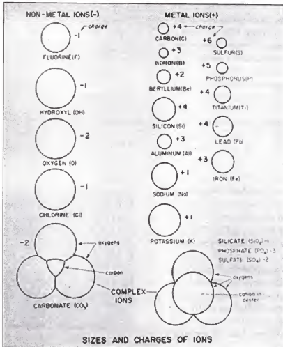
Fig. 6-30. Sizes and charges of ions.
