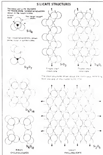
Fig. 6-49. Silicon makes forms and relationships.
