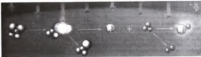
Fig. 3-5. Ozone reaction in molecules.
