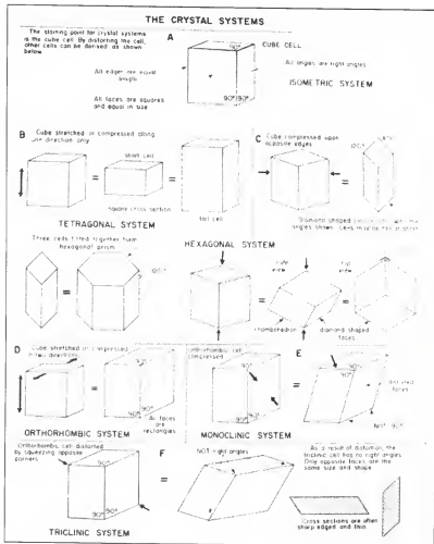
Fig. 6-34. Crystal systems.
