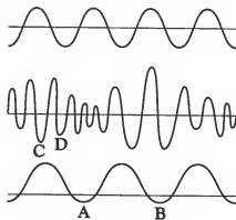
Fig. 2-29. Sample sine waves.
