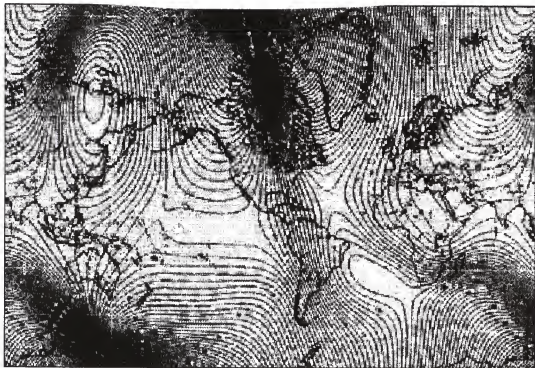
Fig. 2-44. Sample of complex model of Earth's main magnetic field, generated by the USGS for the year 1995.
