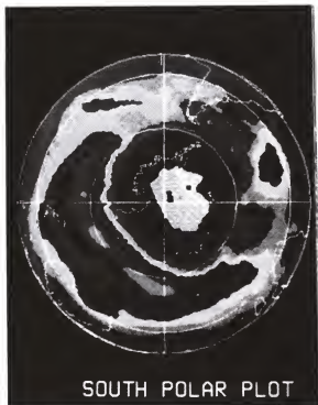
Fig. 3-4. Ozone hole above the South Pole.
