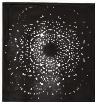
Fig. 6-28. Atomic pattern of a beryl crystal.
