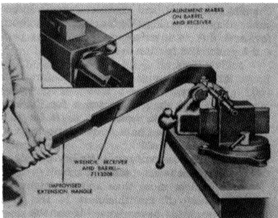
Figure 91. Assembling barrel to receiver.
