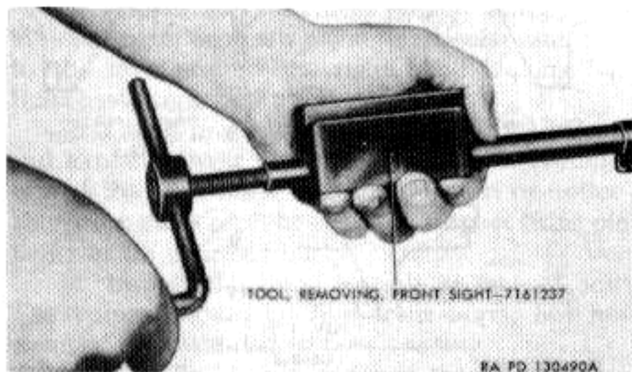
Figure 63. Removing front sight.
