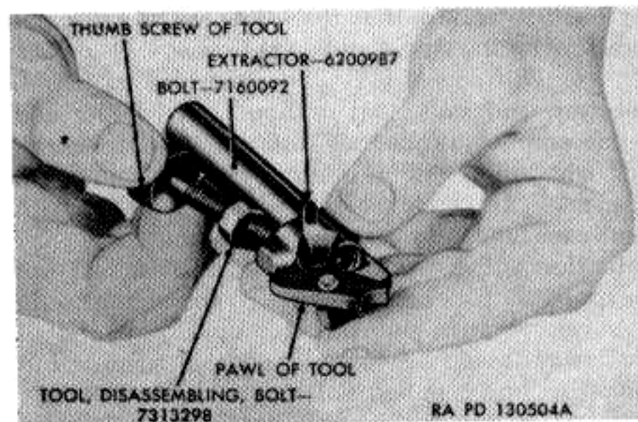
Figure 60. Disassembling bolt.
