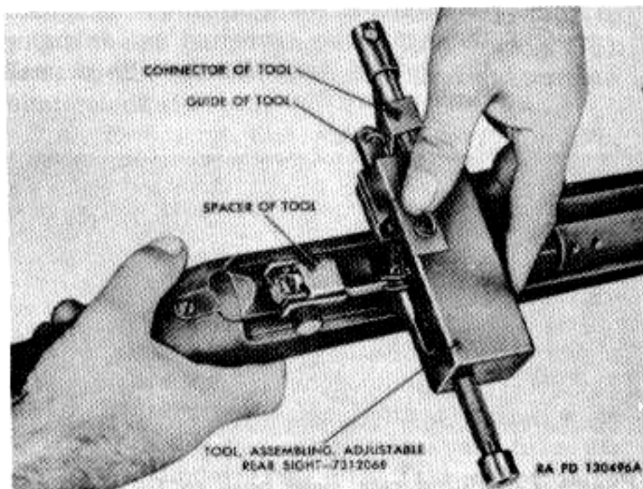
Figure 69. Rear sight assembling tool with spacer.
