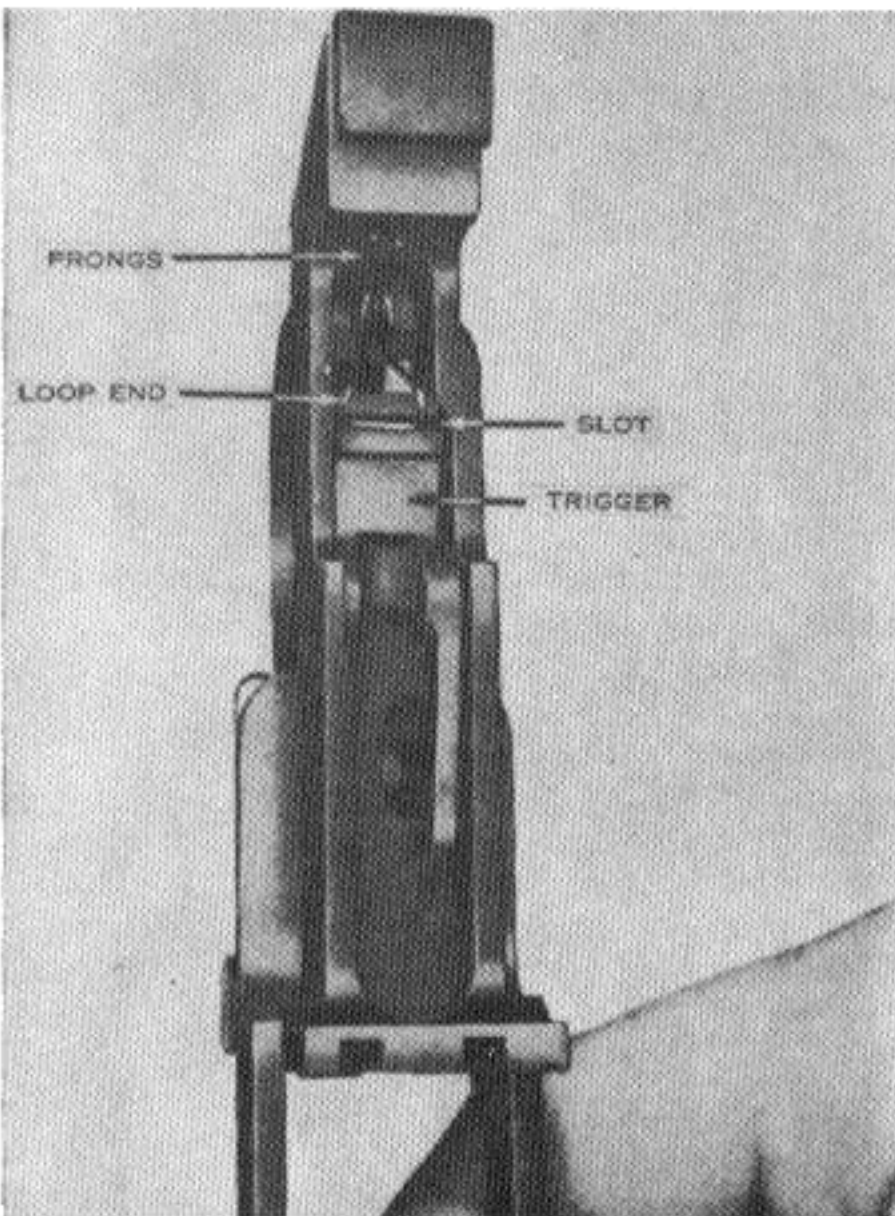
Figure 28. Trigger spring in proper position.
