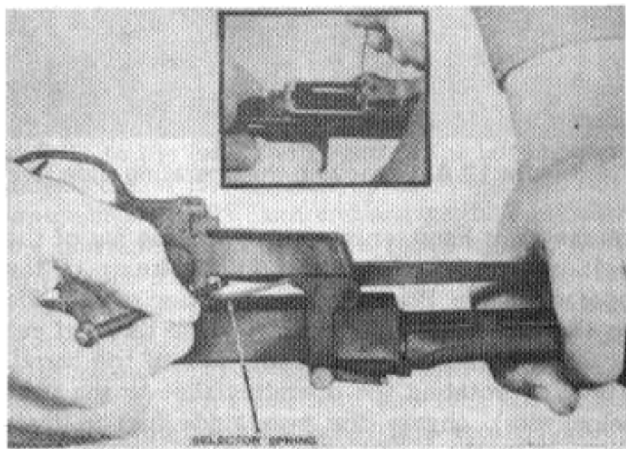
Figure 8. Removing the selector spring.
