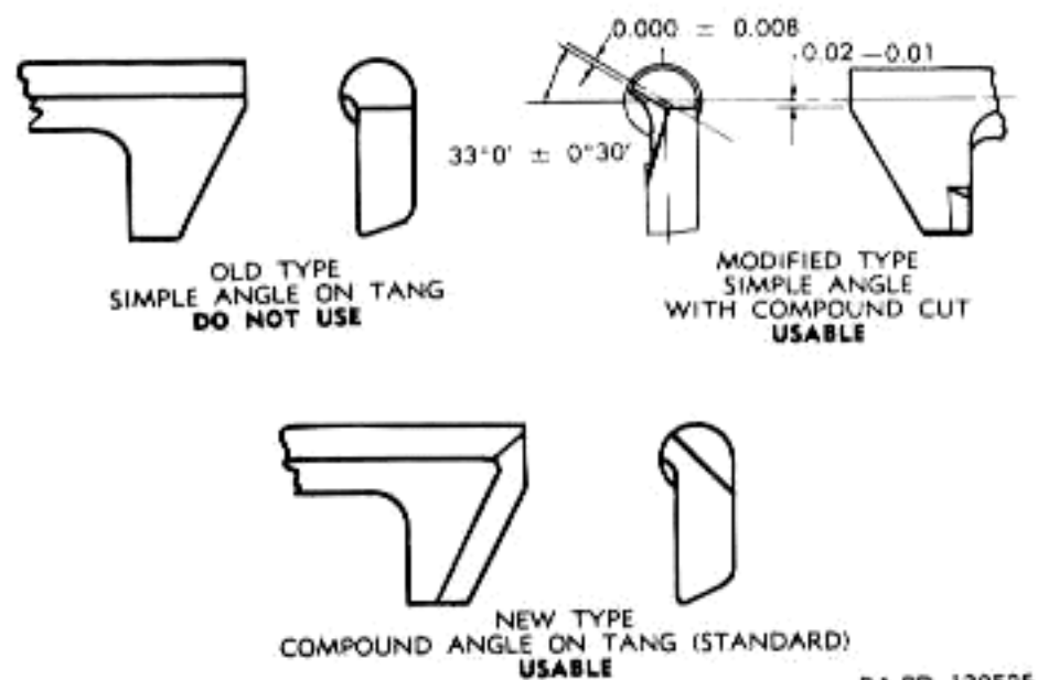
Figure 62. Firing pin 6200976.
