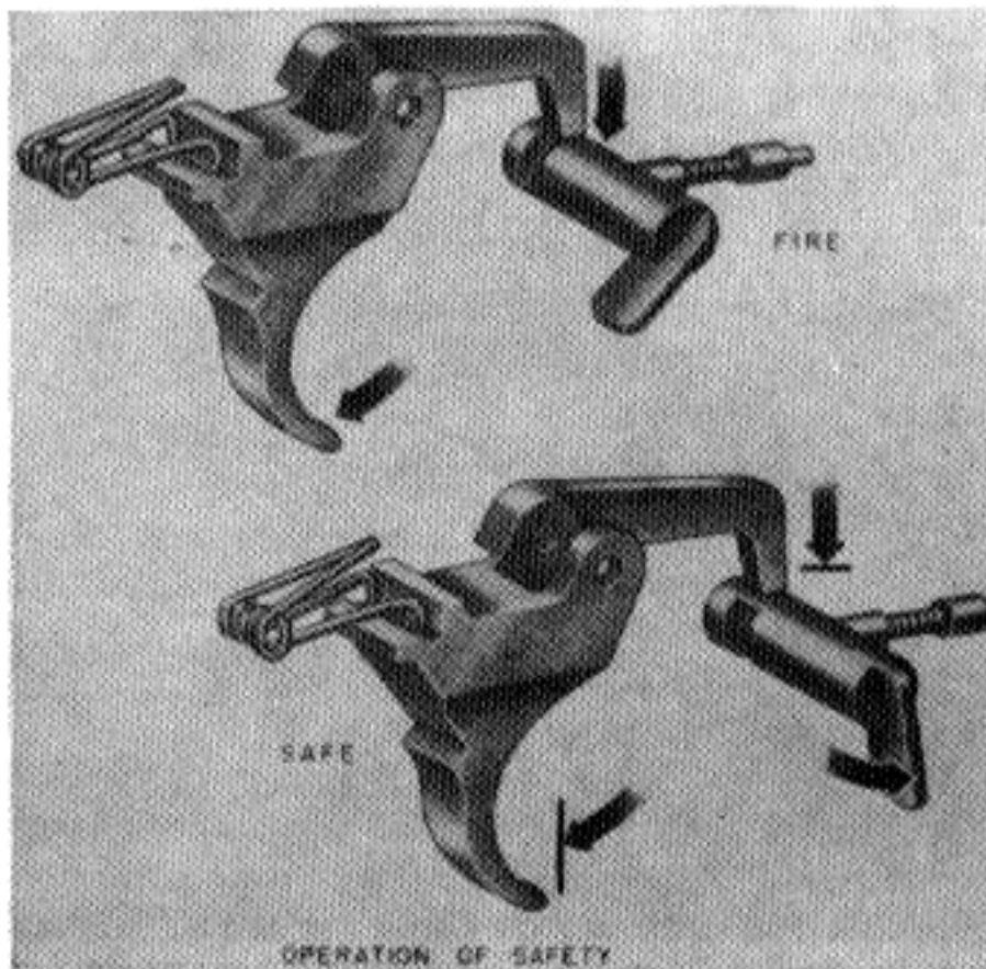
Figure 43. How the safety works.
