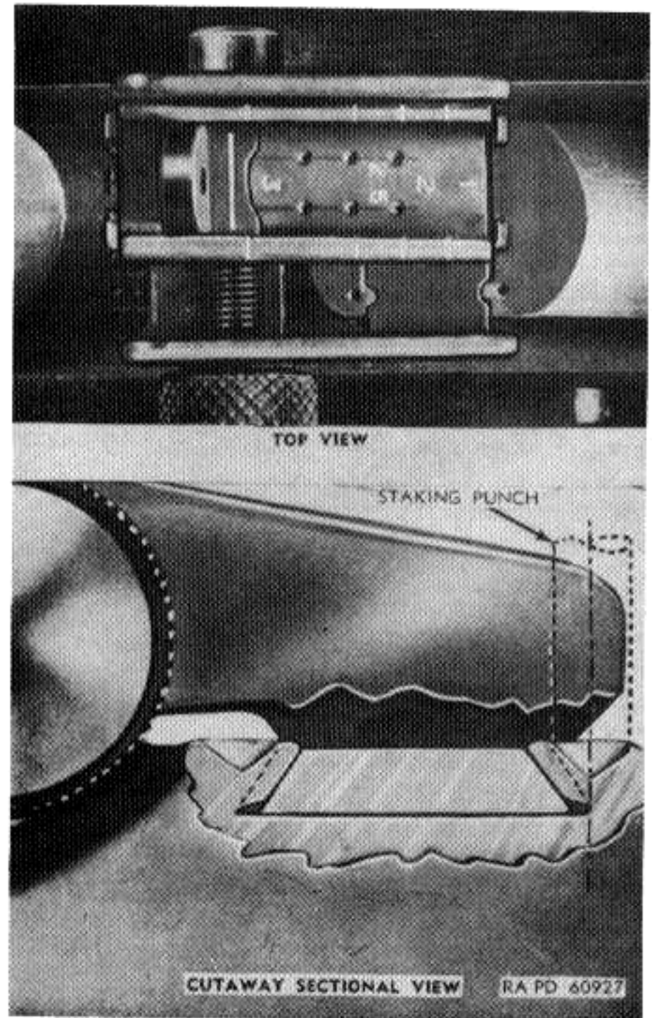
Figure 73. Rear sight showing staking.
