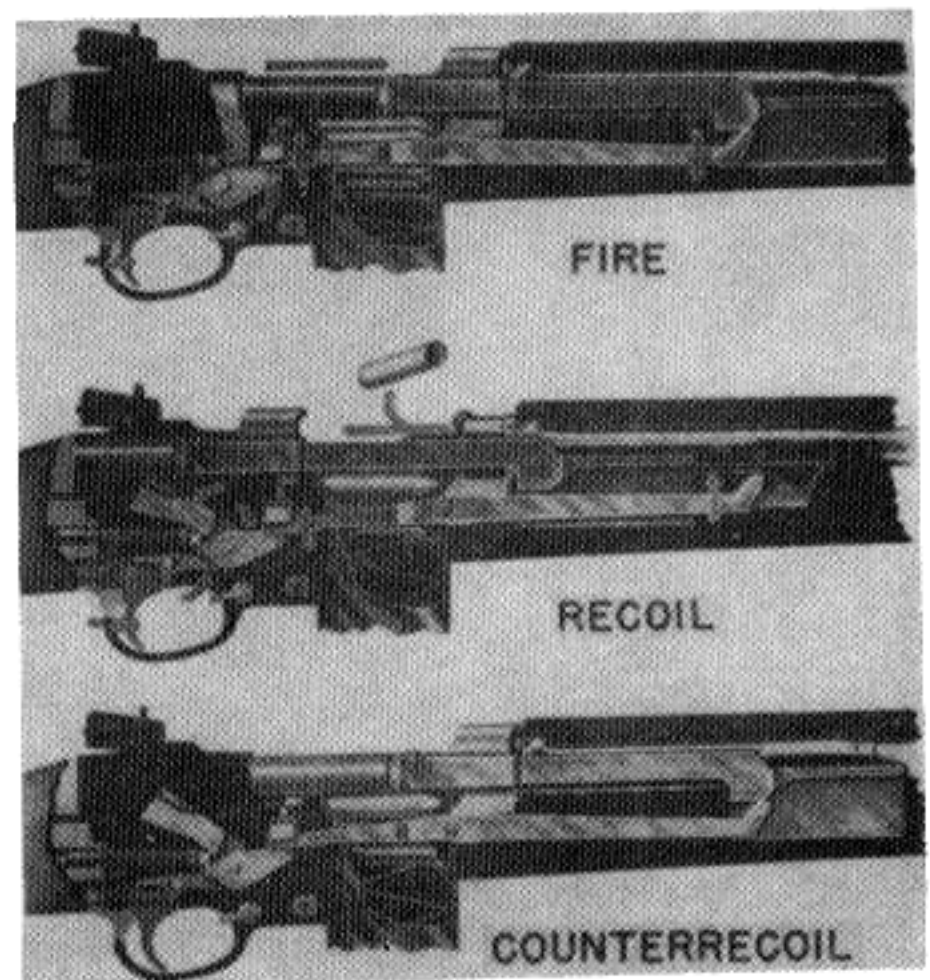
Figure 42. Functioning of operating parts (automatic setting).
