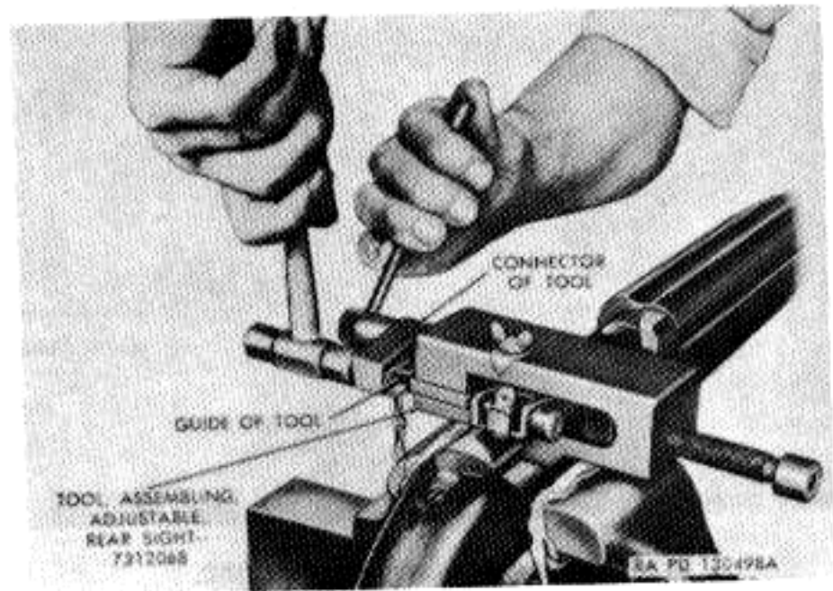
Figure 68. Removing adjustable rear sight.
