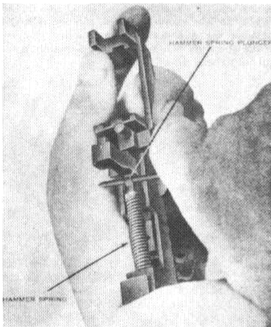
Figure 19. Removing the hammer spring and hammer spring plunger.
