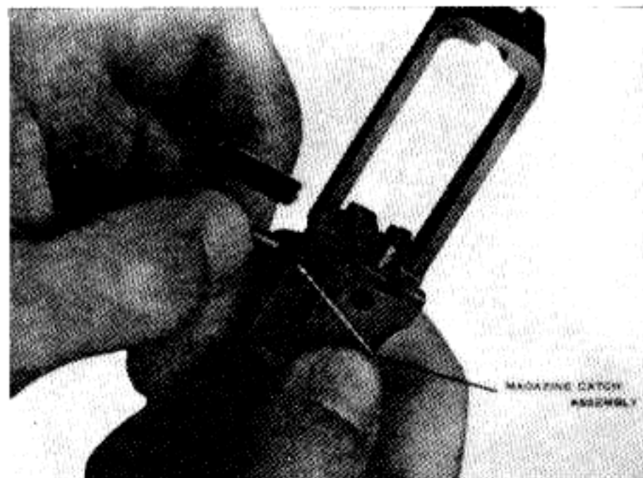
Figure 23-B. Removing the magazine catch plunger assembly.
