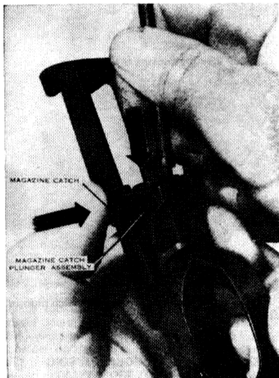
Figure 26. Replacing the magazine catch.
