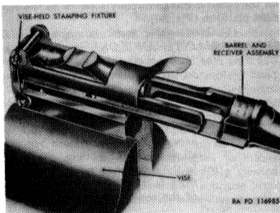
Figure 88. Vise-held stamping fixture with barrel and receiver assembly in place.
