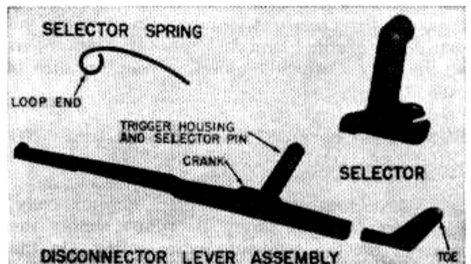
Figure 34. Trigger housing group parts.
