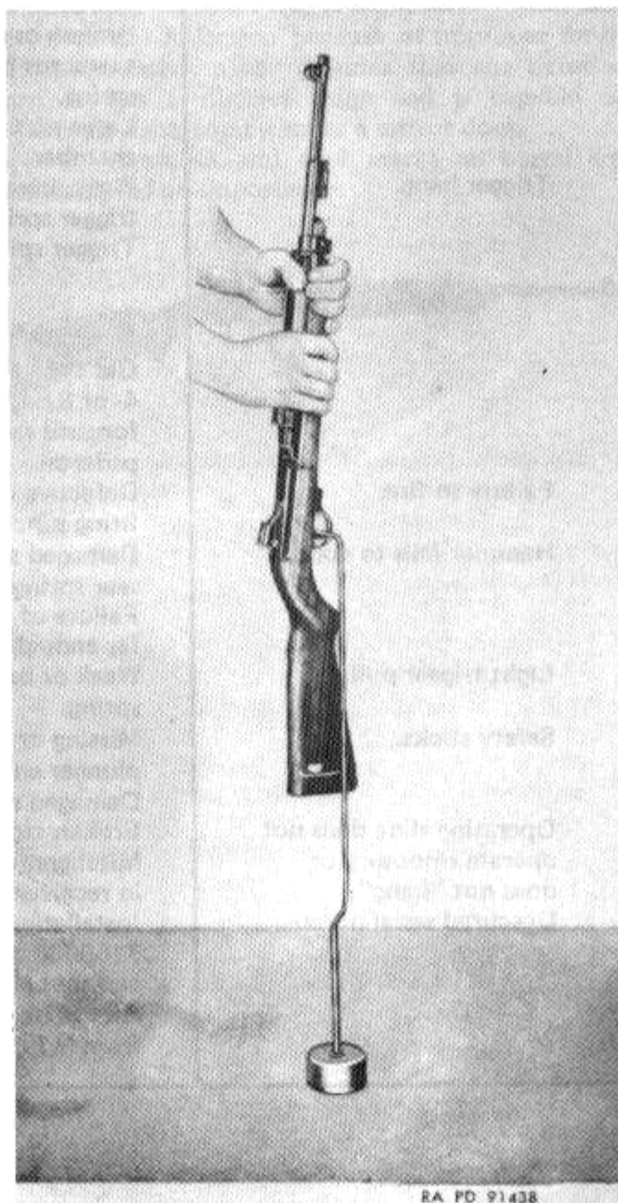
Figure 43c. Testing trigger pull.
