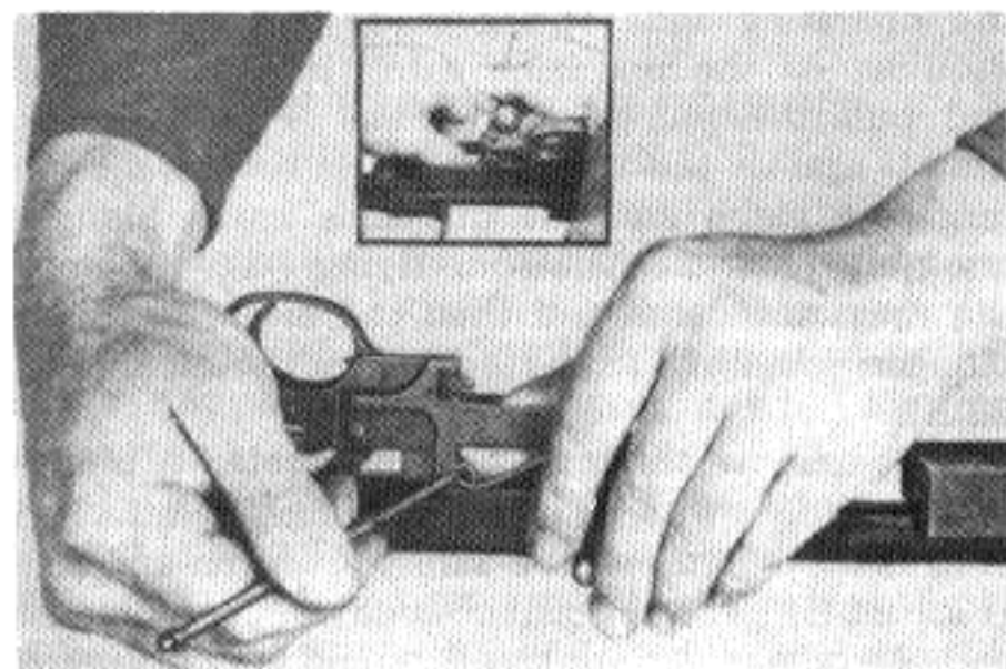
Figure 17. Replacing the selector spring.
