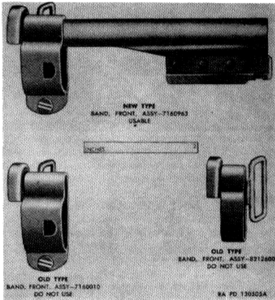
Figure 81. Front band assemblies.
