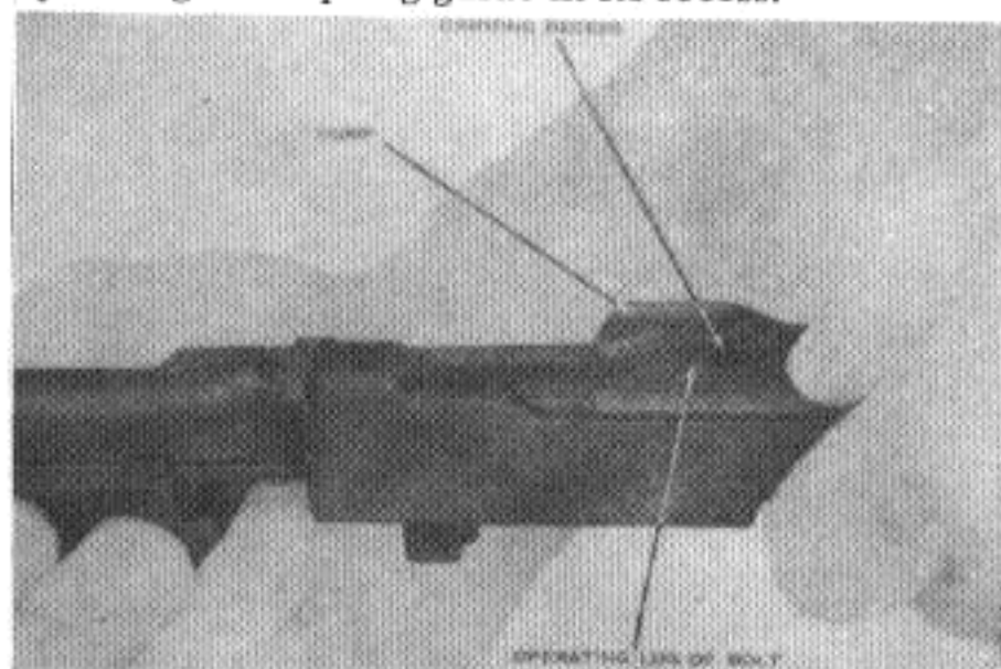
Figure 15-A. Replacing the operating slide.
