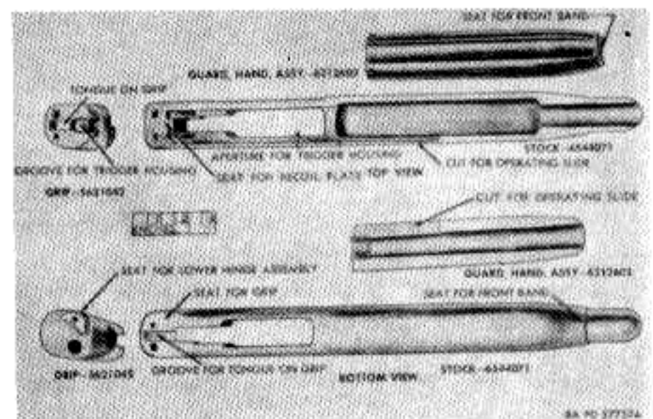
Figure 107. Stock, hand guard and grip for carbine M1A1.
