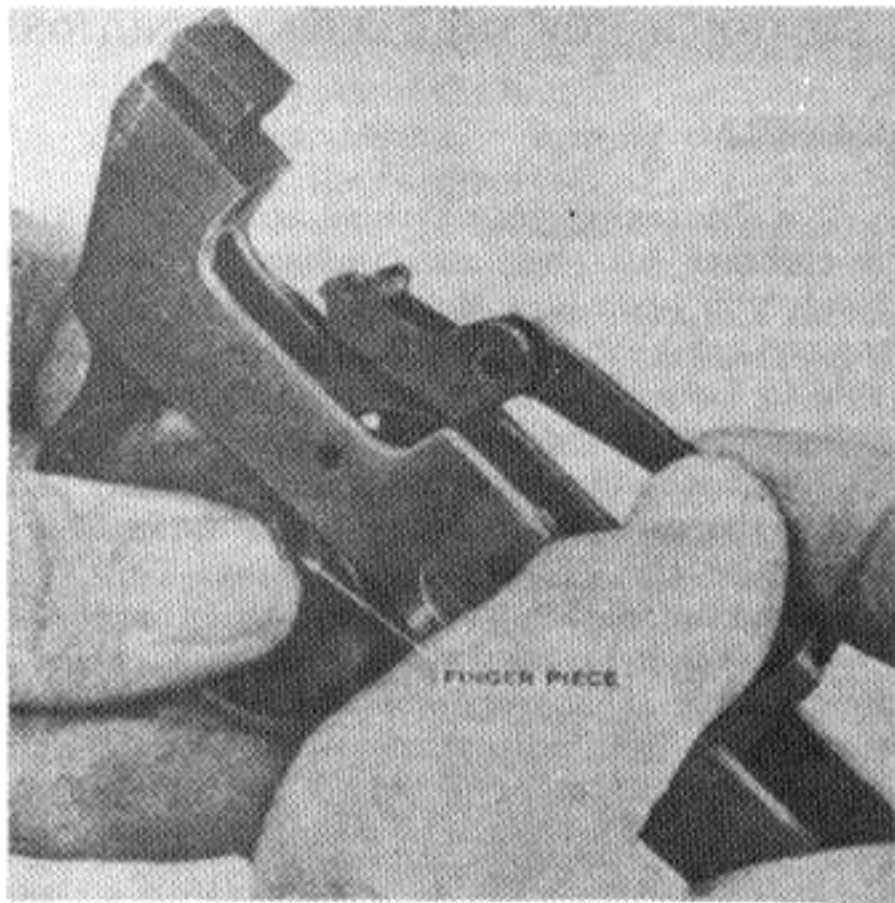
Figure 27. Replacing the trigger.
