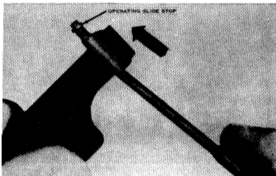
Figure 32. Removing the operating slide stop.
