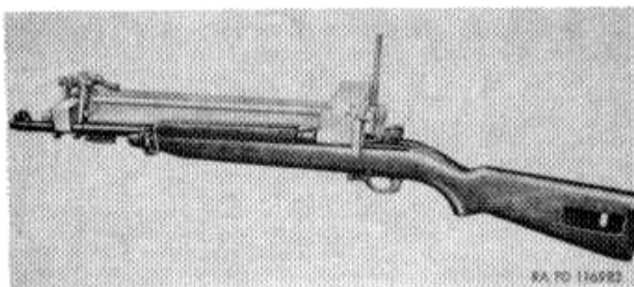
Figure 89. Carbine clamped in bench-mounted stamping fixture.
