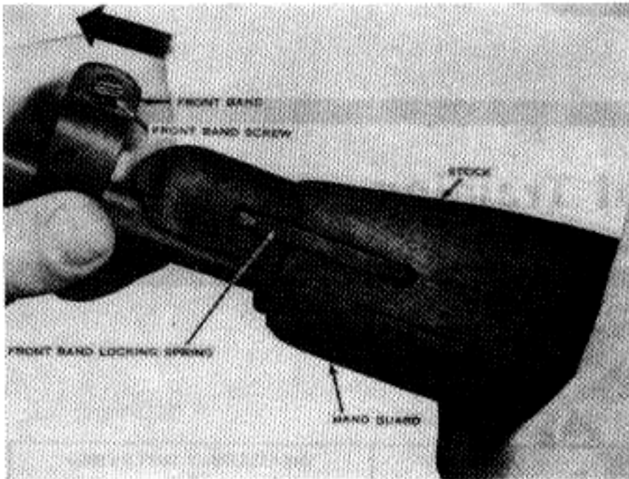
Figure 4. Sliding the front band forward.
