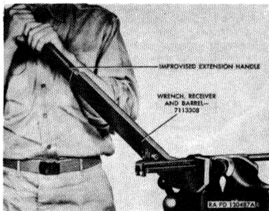
Figure 76. Removing barrel from receiver.
