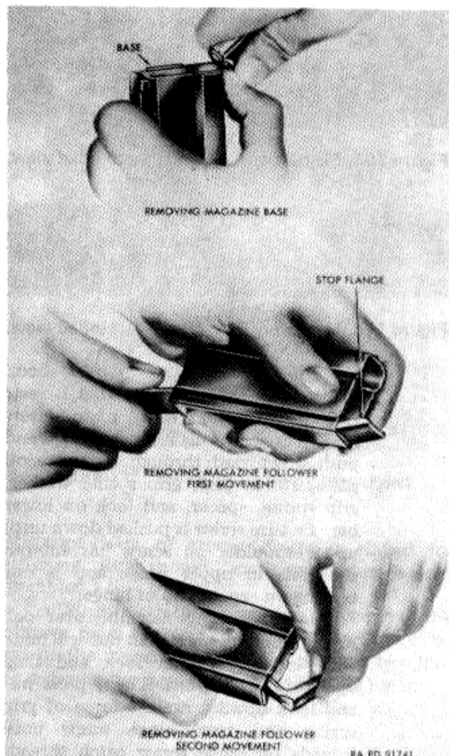
Figure 108. Removing magazine base and follower.
