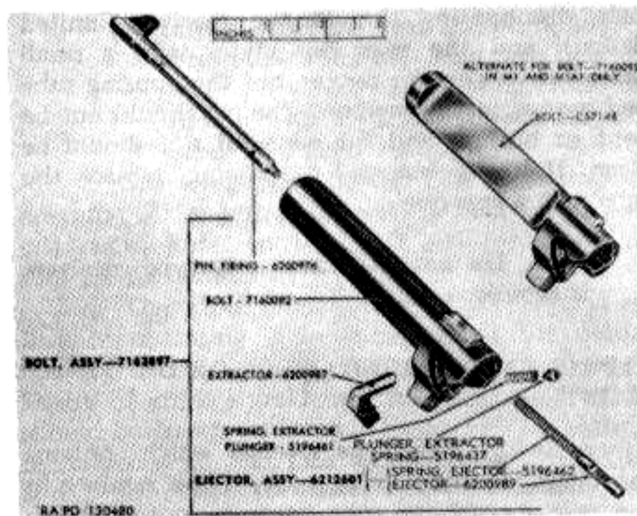
Figure 59. Bolt assembly.
