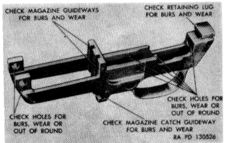
Figure 47. Trigger housing inspection points.
