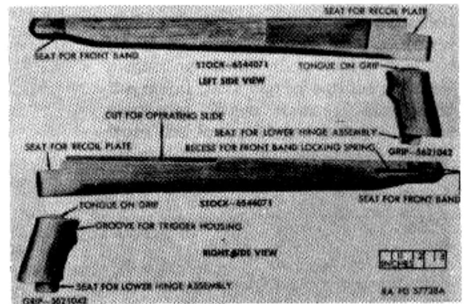
Figure 106. Stock and grip for carbine M1A1.
