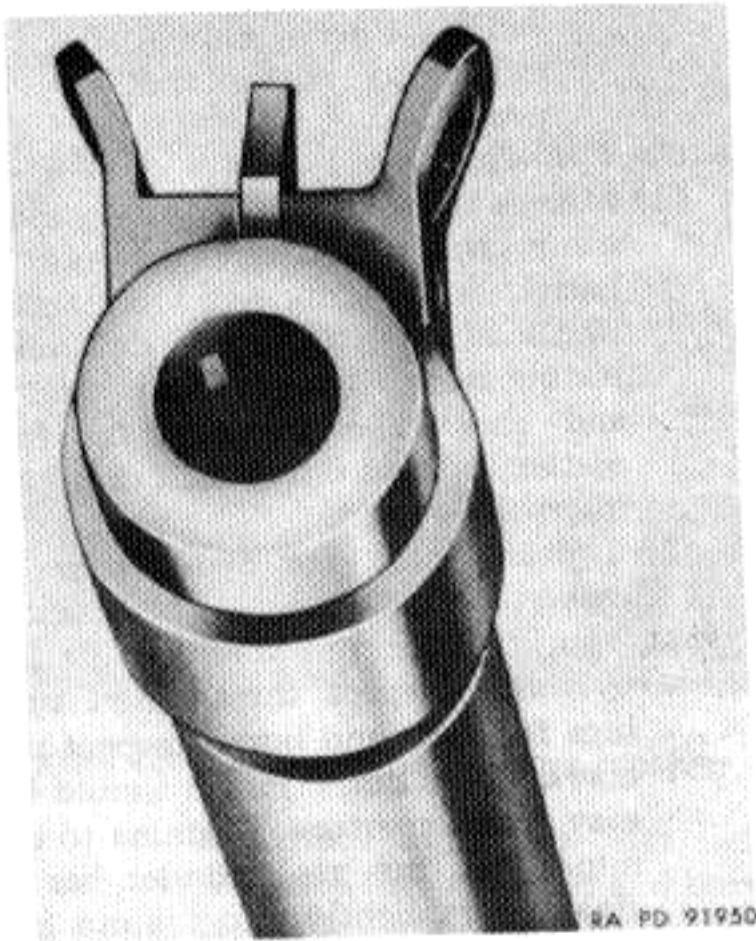
Figure 79. Muzzle end of barrel showing counterbore.
