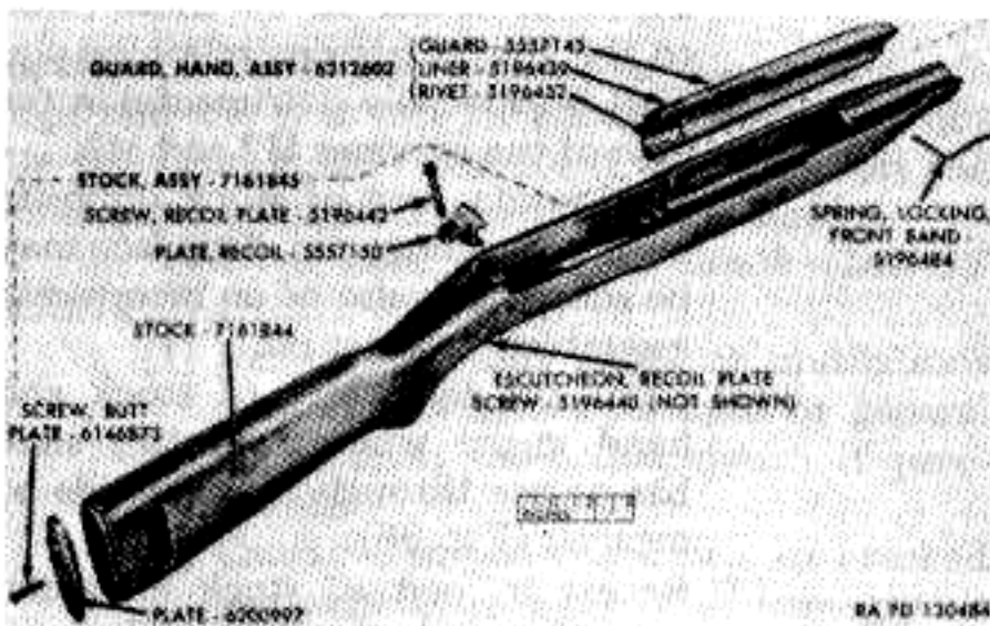
Figure 94. Stock and guard assemblies — carbines M1, M2 and M3.
