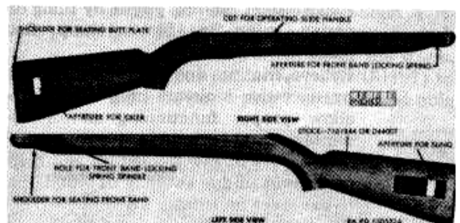
Figure 95. Stock showing apertures — carbine M1.
