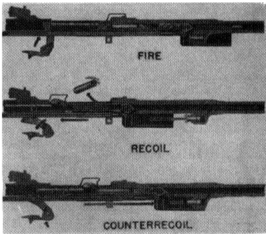
Figure 40. Action of the gas.
