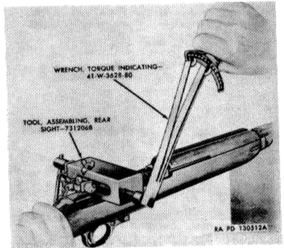
Figure 70. Moving rear sight in place with torque wrench.
