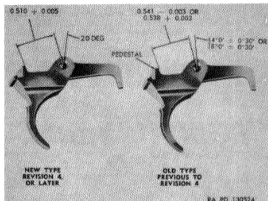
Figure 51. Trigger 6200988.
