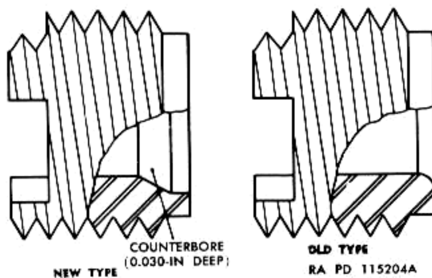
Figure 43e. Piston nut 5196436.
