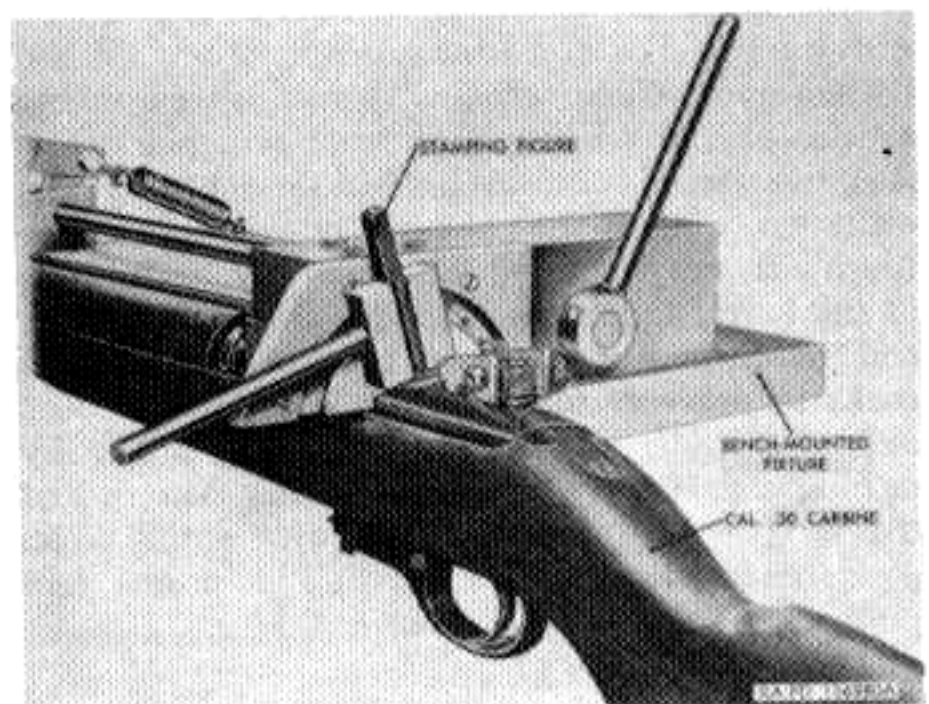
Figure 90. Bench-mounted stamping fixture with carbine and stamping figure in place.
