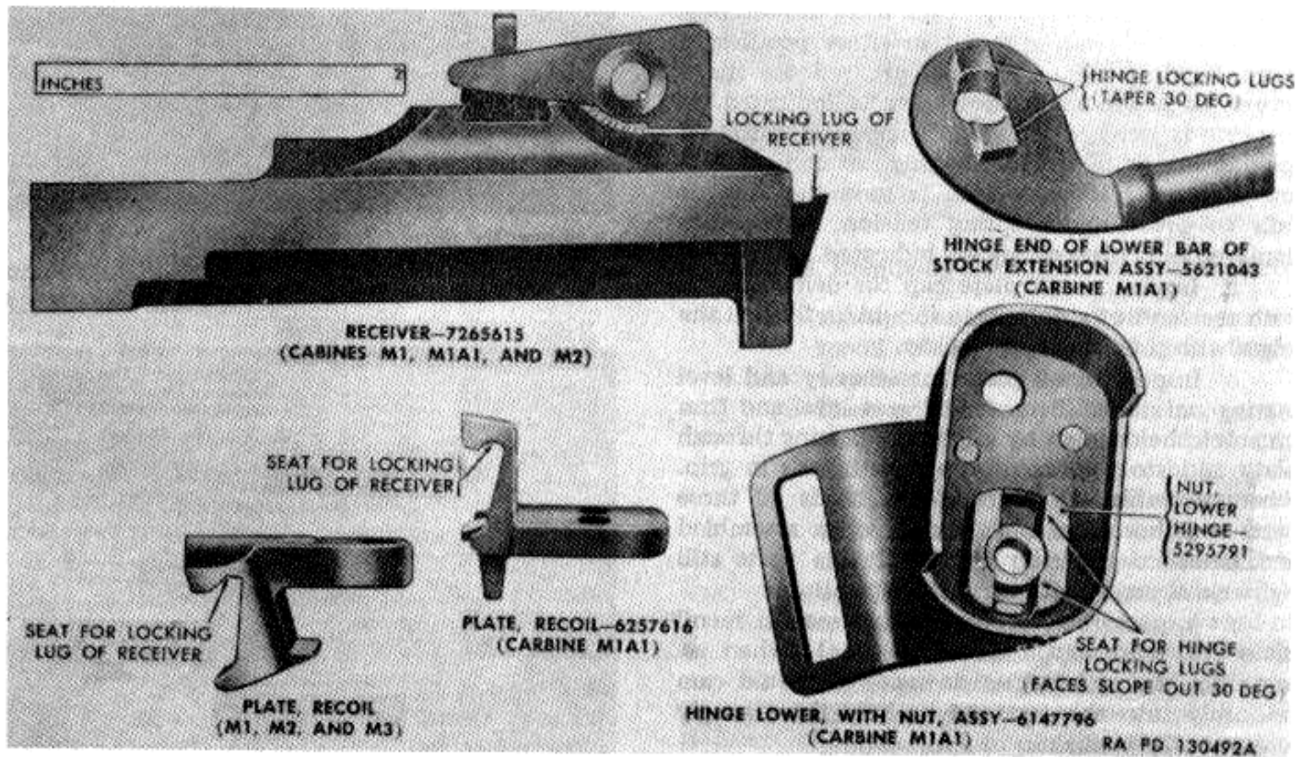
Figure 104. Important wearing surfaces.
