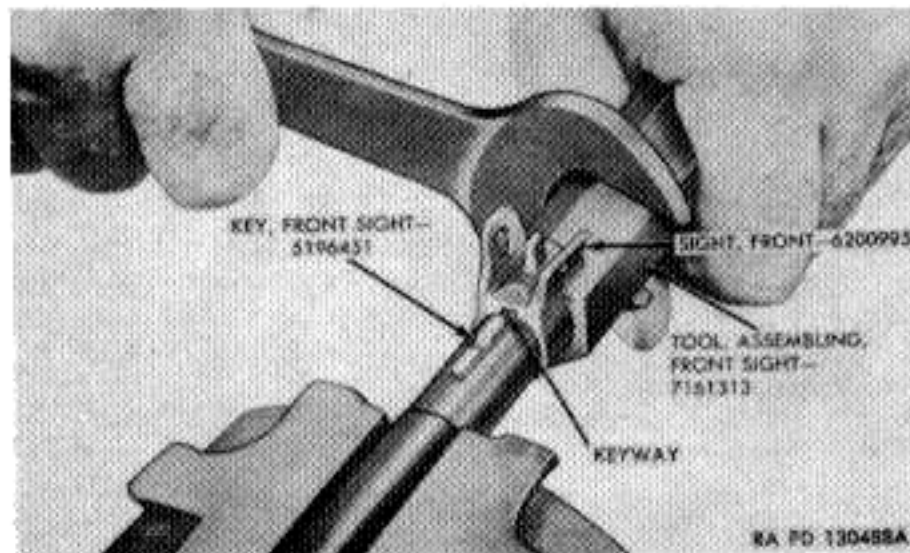
Figure 64. Aligning front sight.
