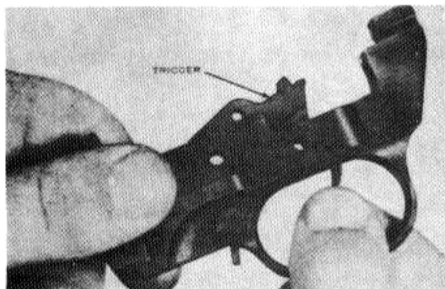
Figure 22. Removing the trigger.
