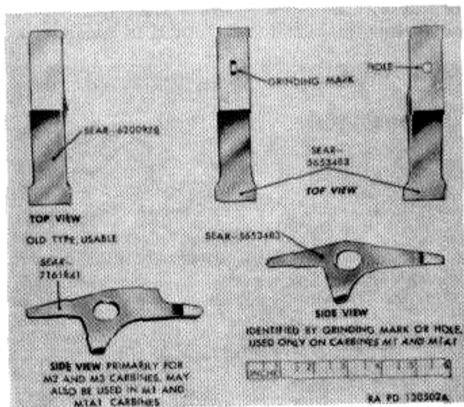
Figure 52. Sears — usable types.
