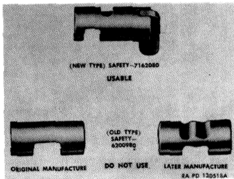
Figure 53. Safeties.
