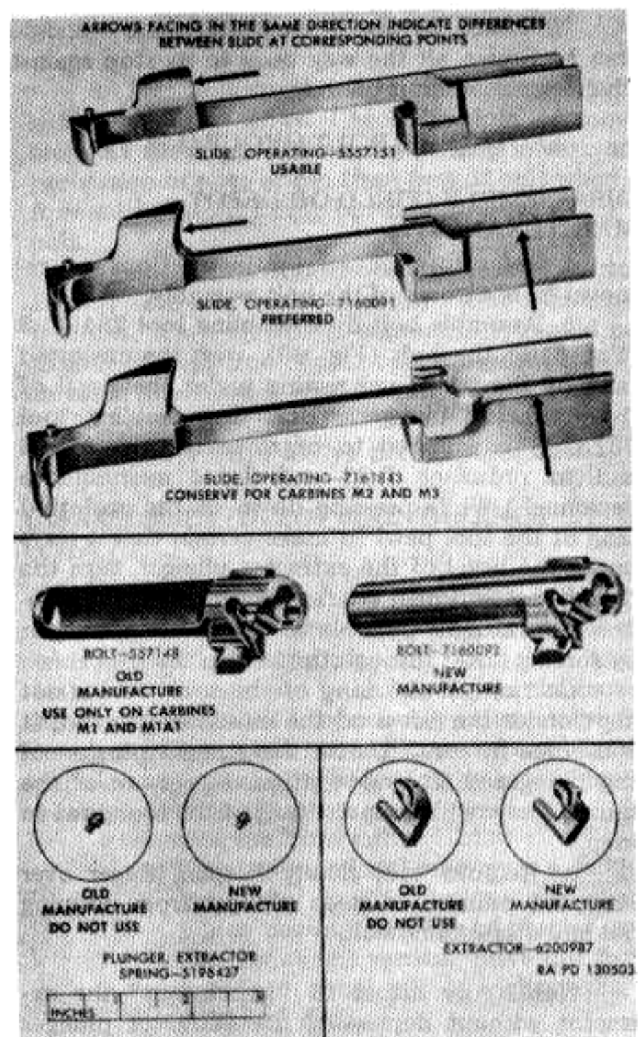
Figure 58. Slide, bolt, extractor and plunger.
