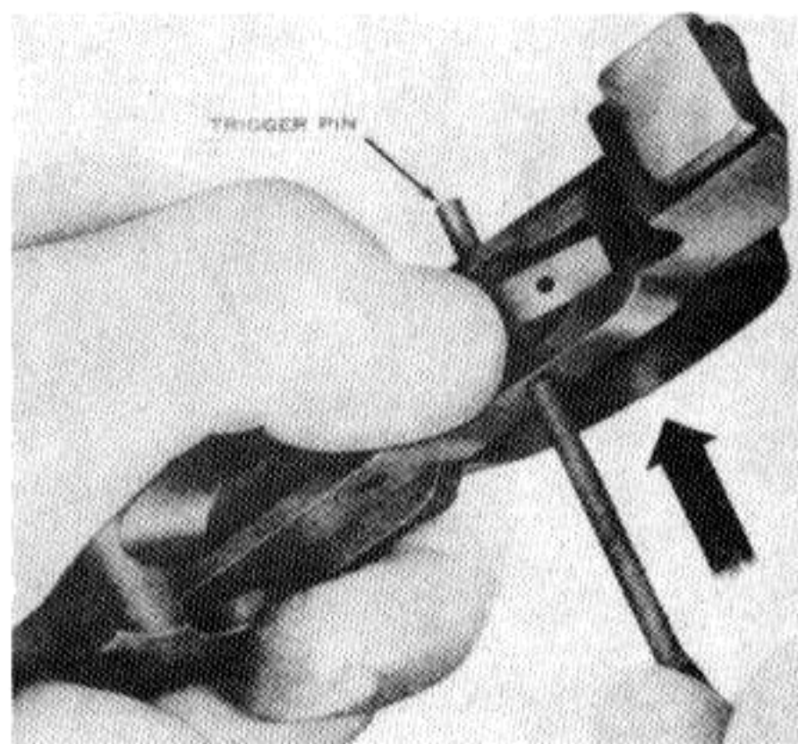
Figure 21. Removing the trigger pin.
