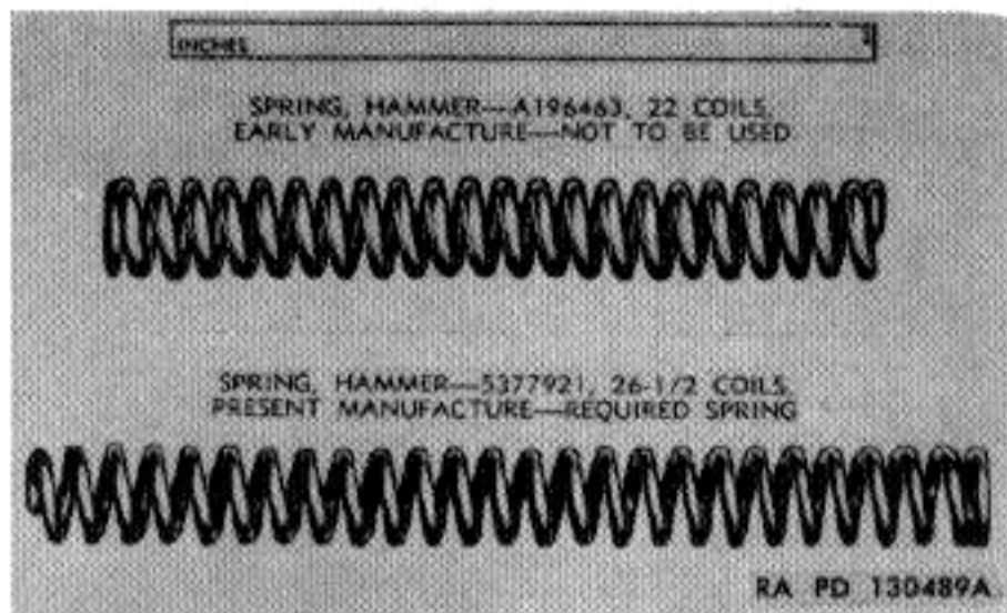
Figure 50. Hammer spring—early and recent design.
