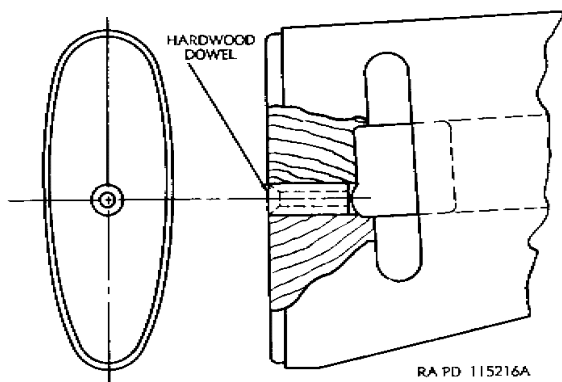
Figure 102. Repair for stripped screw hole.
