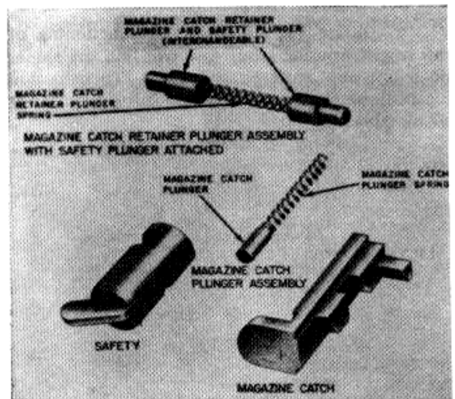
Figure 36. Trigger housing group parts.
