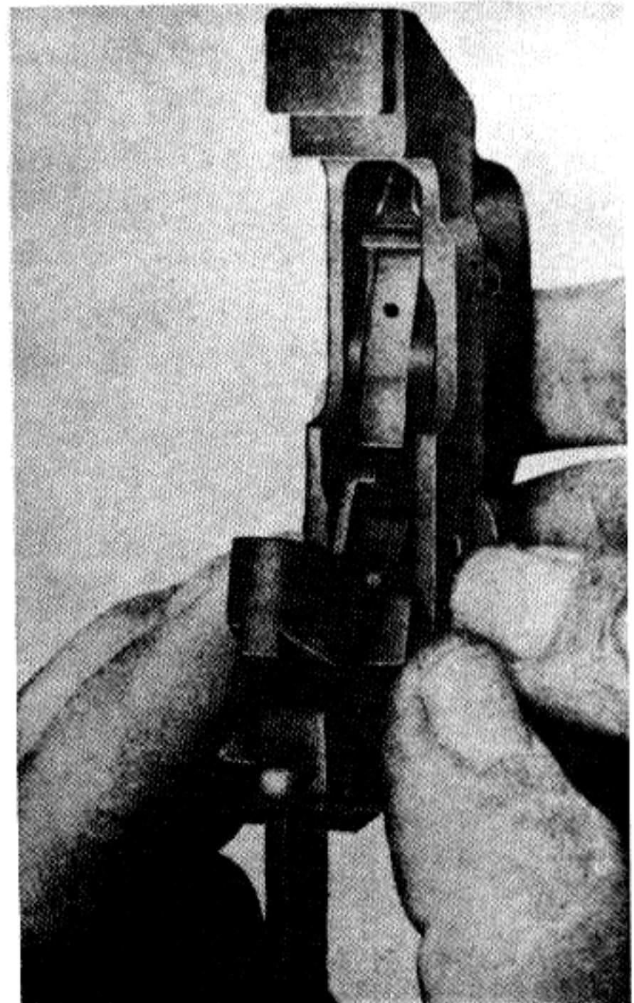
Figure 31. Replacing the hammer.
