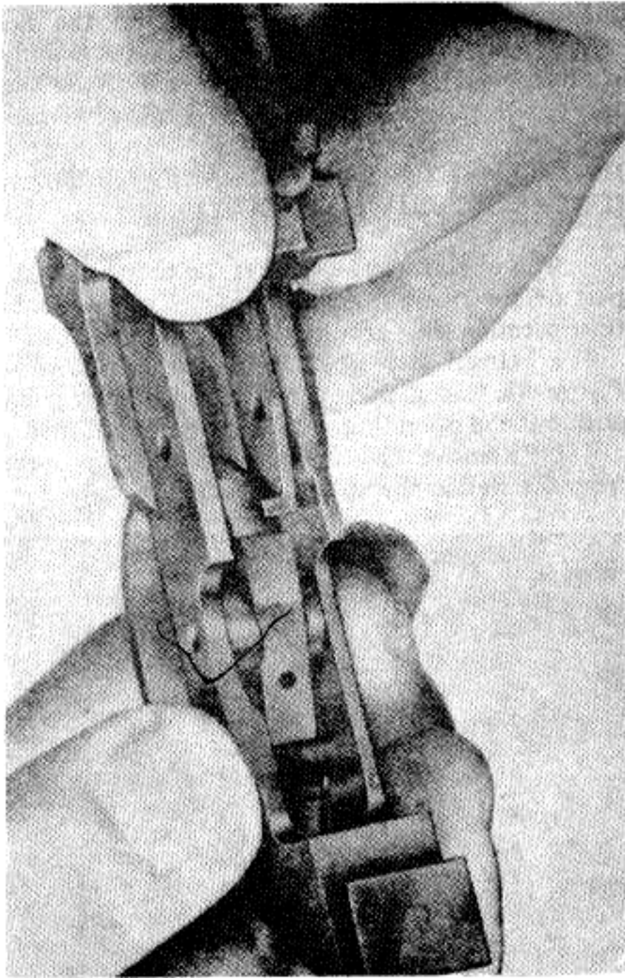
Figure 30. Replacing the disconnecter.
