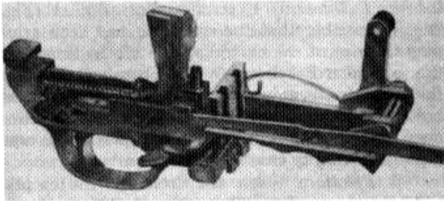
Figure 38. Functioning of trigger housing group.
