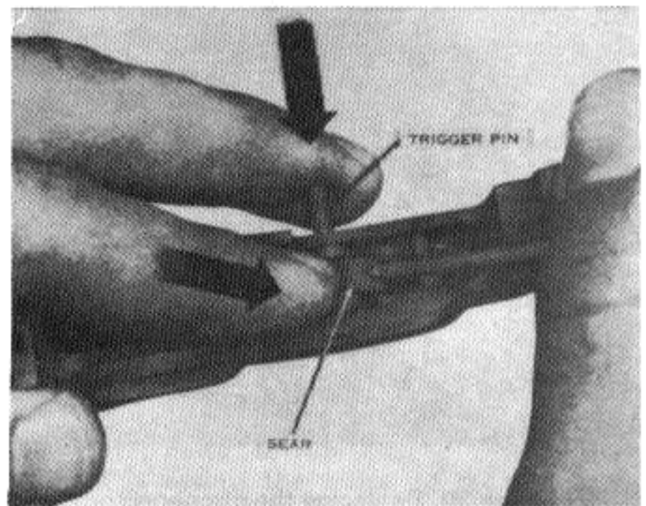
Figure 29. Replacing the trigger pin.
