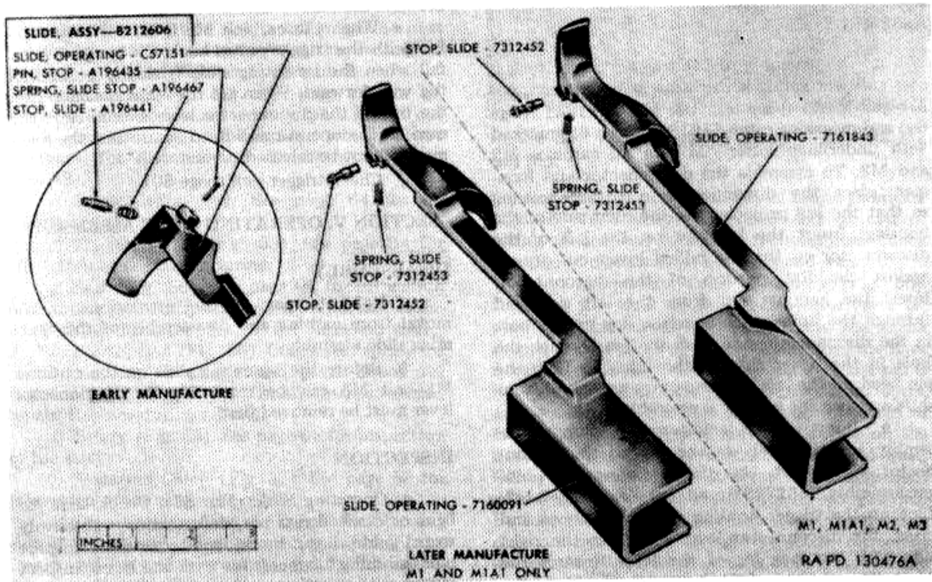
Figure 57. Operating slide assembly.
