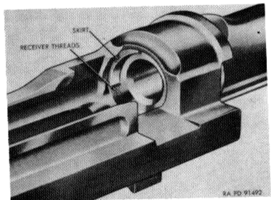
Figure 80. Breech and barrel showing new type skirt.
