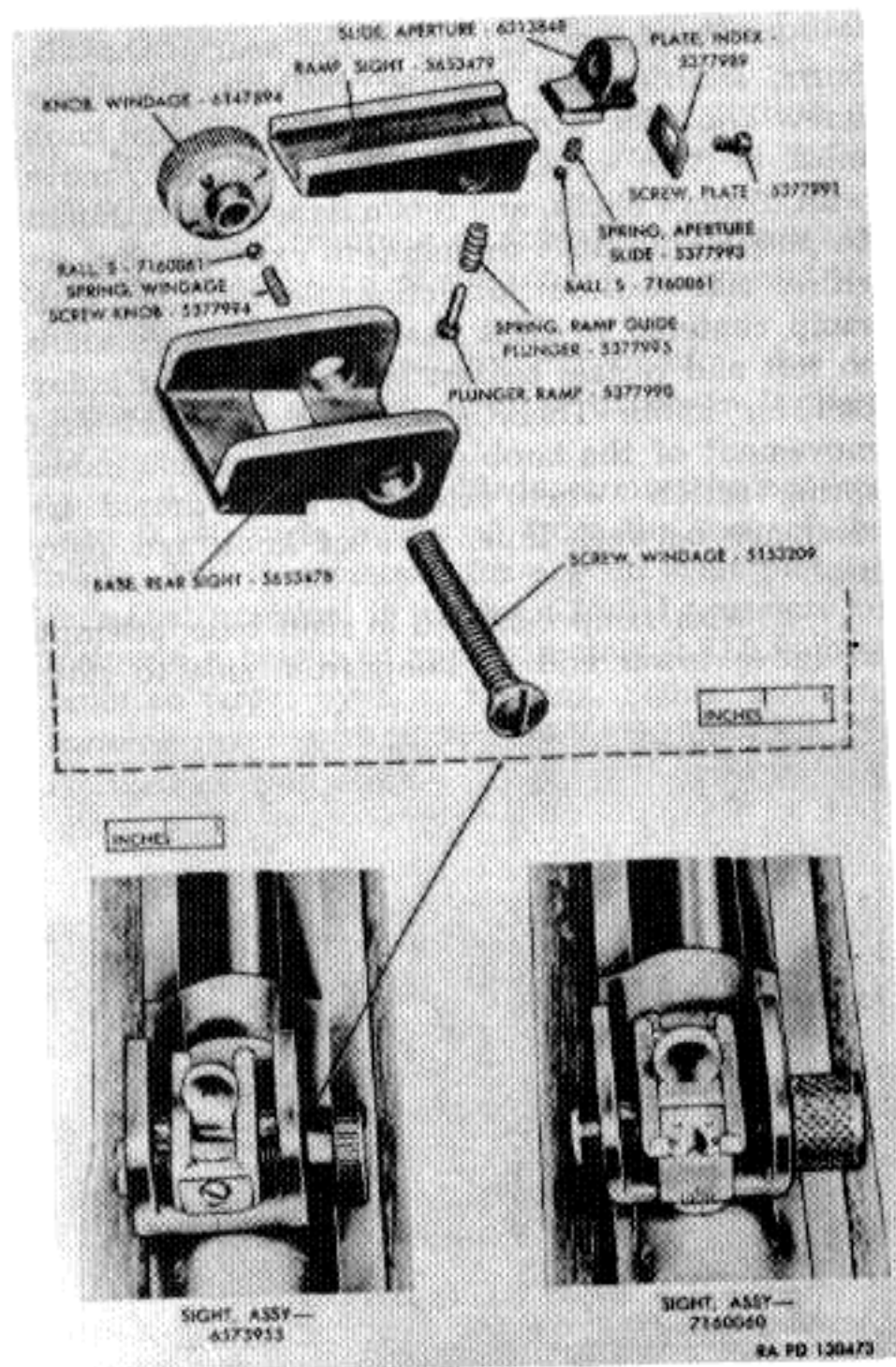
Figure 67. Adjustable rear sight assembly for M1, M1A1 and M2 carbines.
