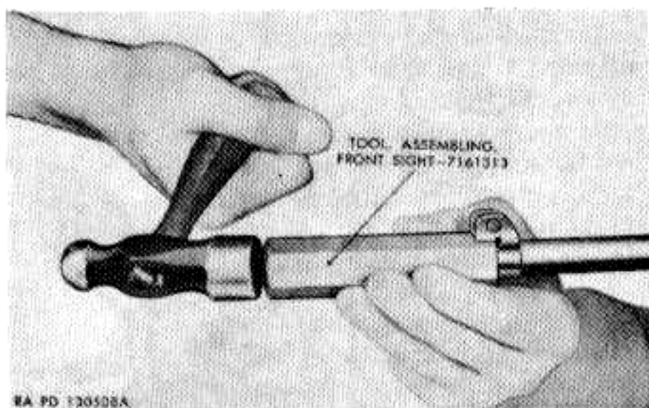
Figure 65. Installing front sight.
