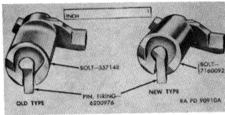
Figure 61. Bolt and firing pin.
