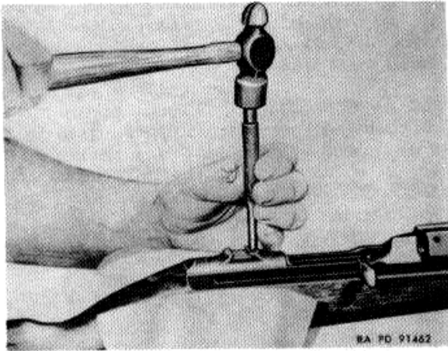
Figure 71. Peening receiver to reduce oversize dovetail slot.
