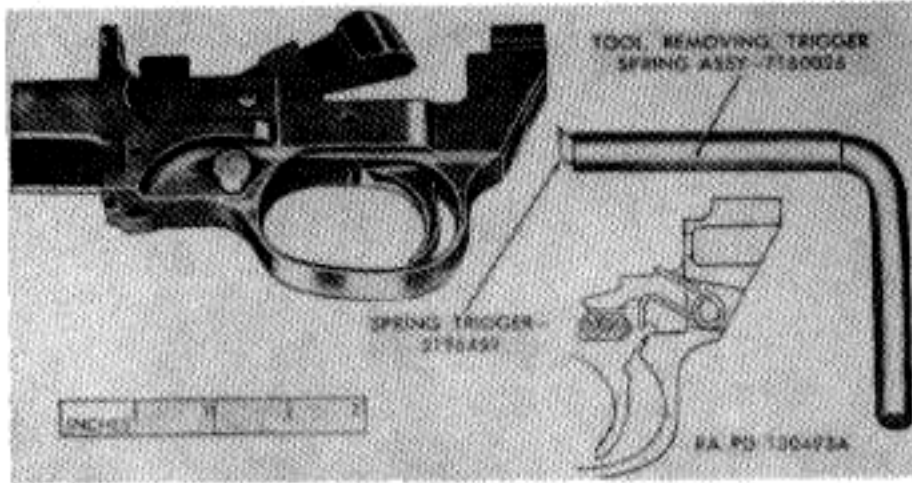
Figure 46. Trigger spring removal and installation.
