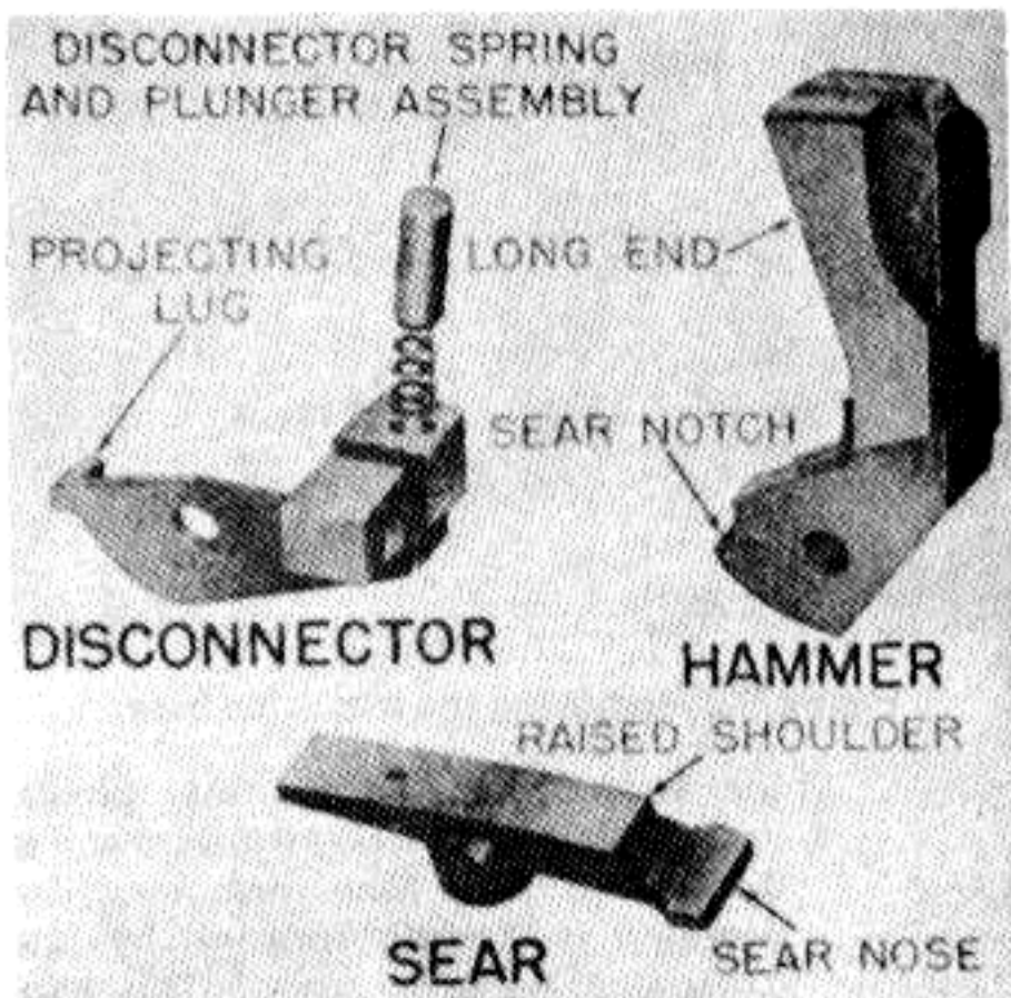
Figure 35. Trigger housing group parts.
