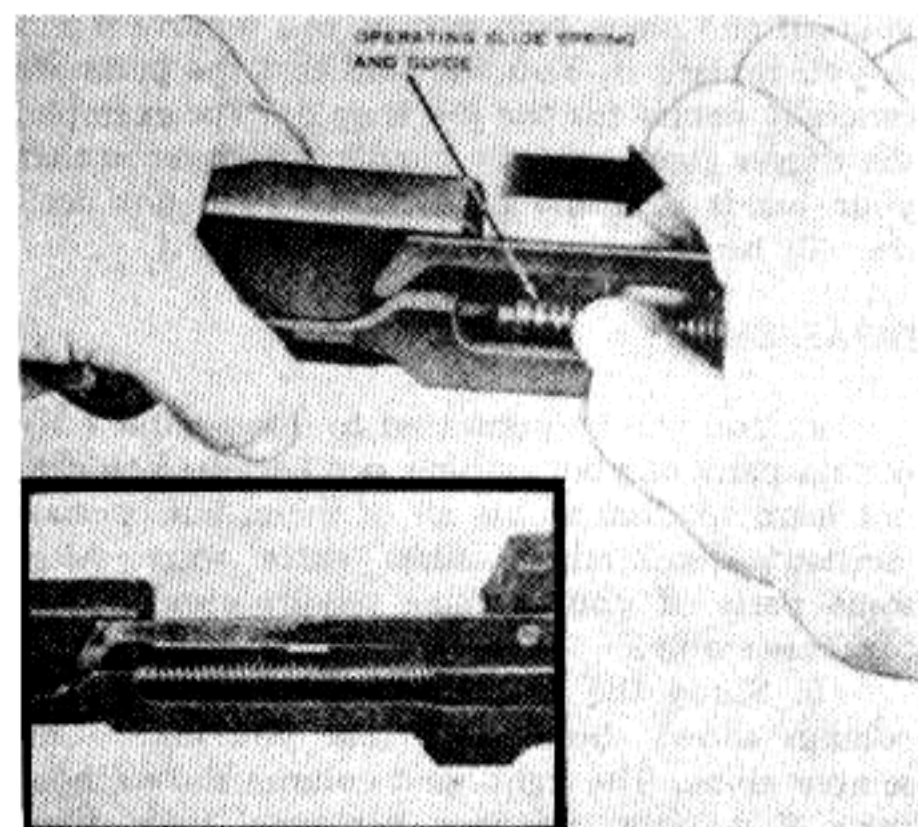
Figure 7. Removing the operating slide spring and guide.
