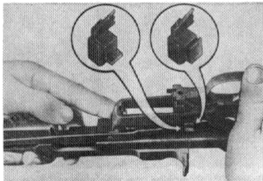
Figure 9. Removing the disconnecter lever assembly.
