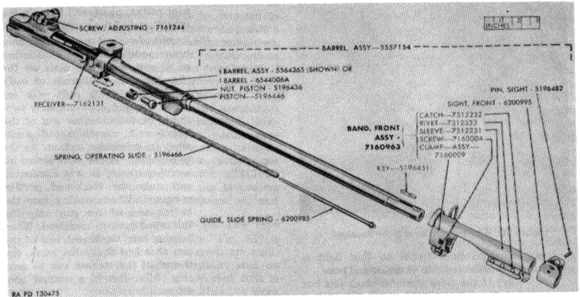
Figure 75. Barrel and receiver group M3 carbine.
