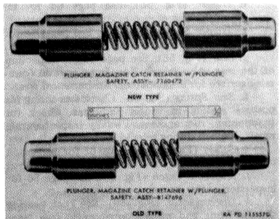
Figure 55. Plunger assemblies for magazine catch and safety.
