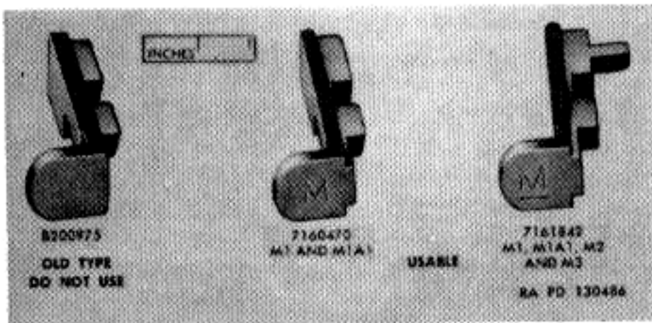
Figure 54. Magazine catches.
