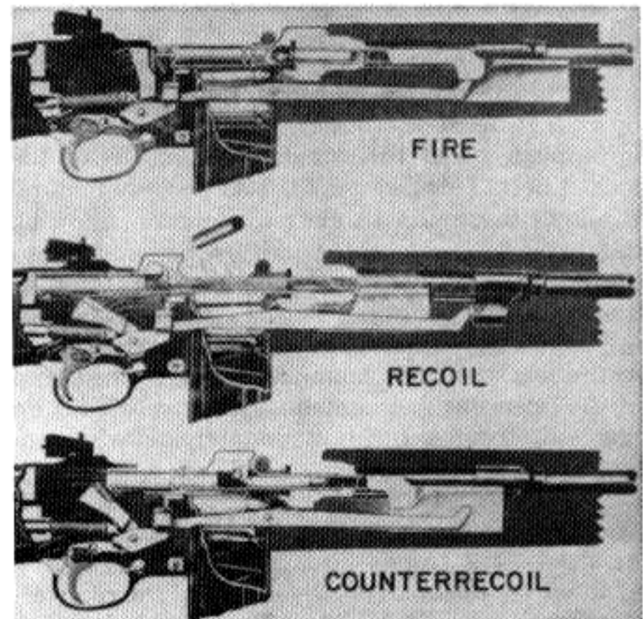
Figure 39. Functioning of operating parts (semi-automatic setting).
