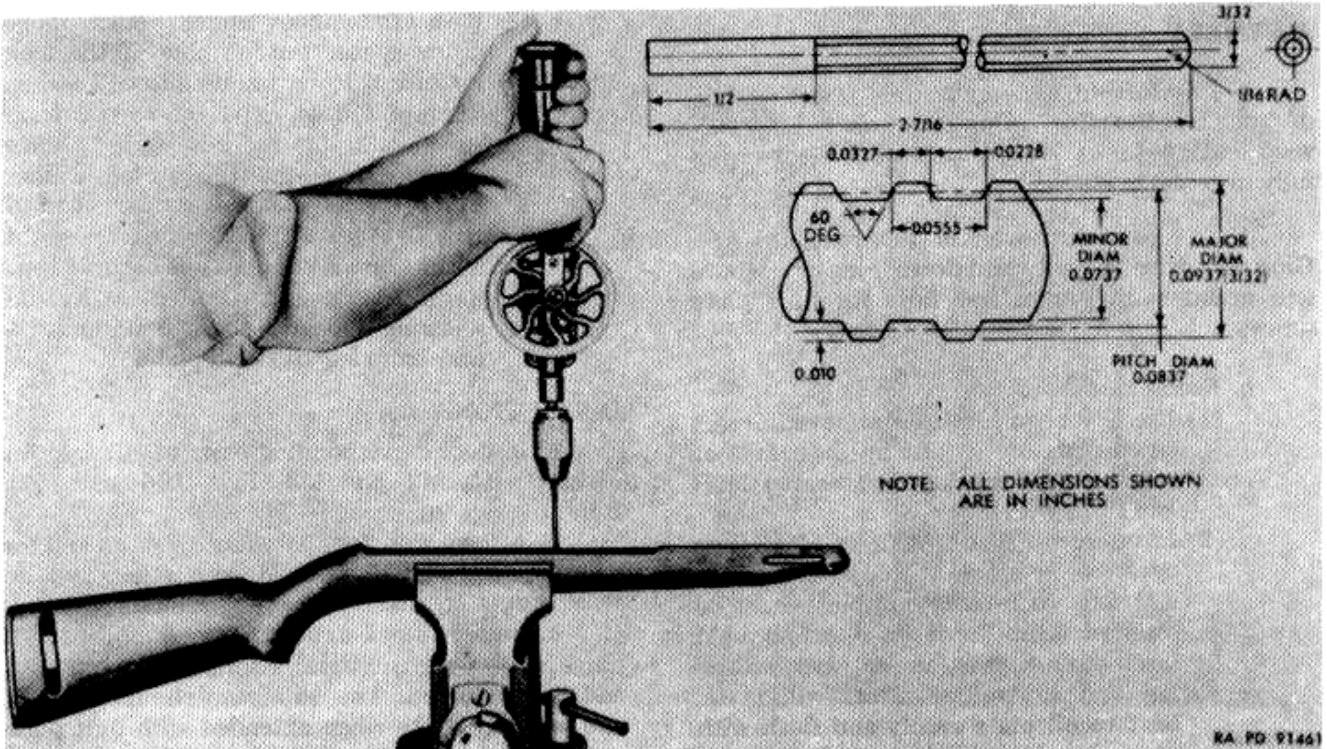
Figure 101. Installing repair screws.
