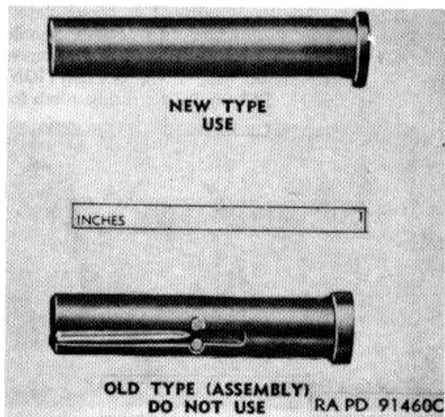
Figure 48. Trigger housing retaining pin.
