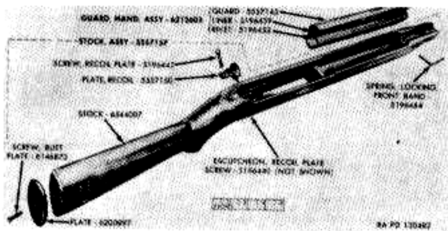
Figure 93. Stock and guard assemblies — carbine M1.
