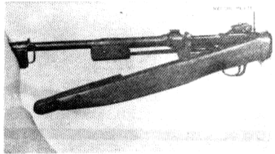
Figure 6. Separating the stock group and the barrel and receiver group.
