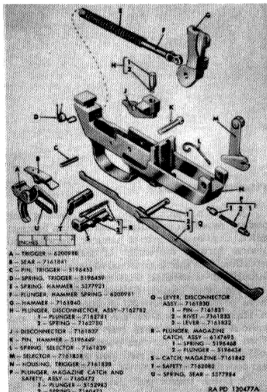
Figure 56. Trigger housing group - carbines M2 and M3.
