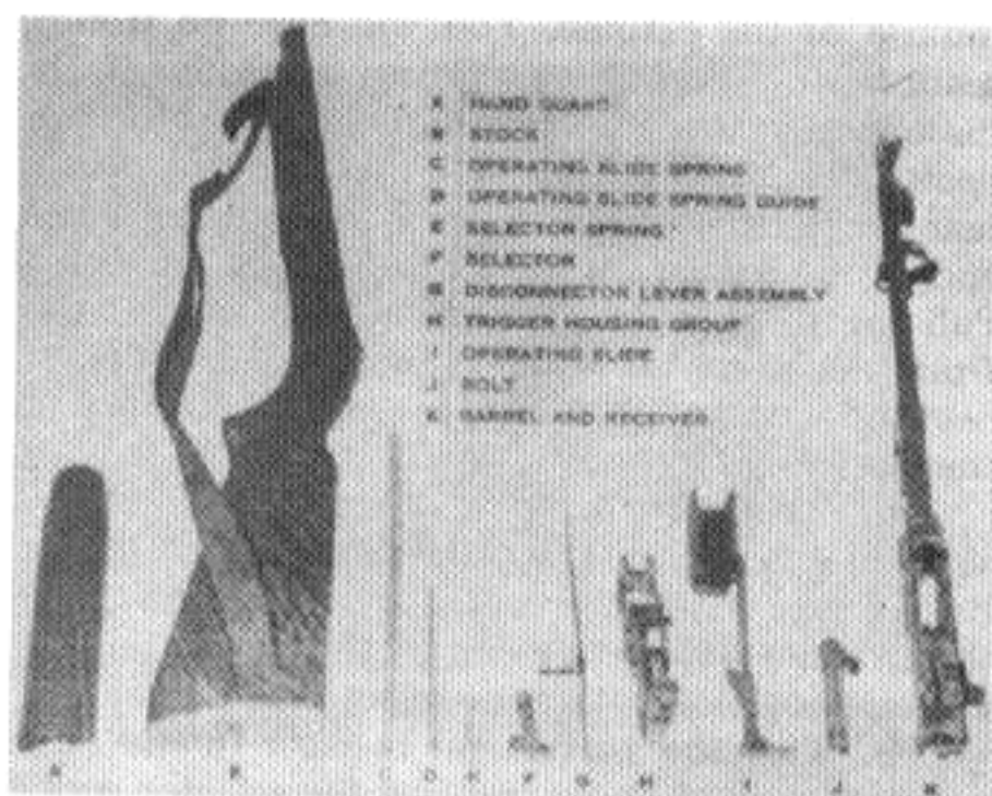
Figure 14. Lay out of parts disassembled during field stripping.
