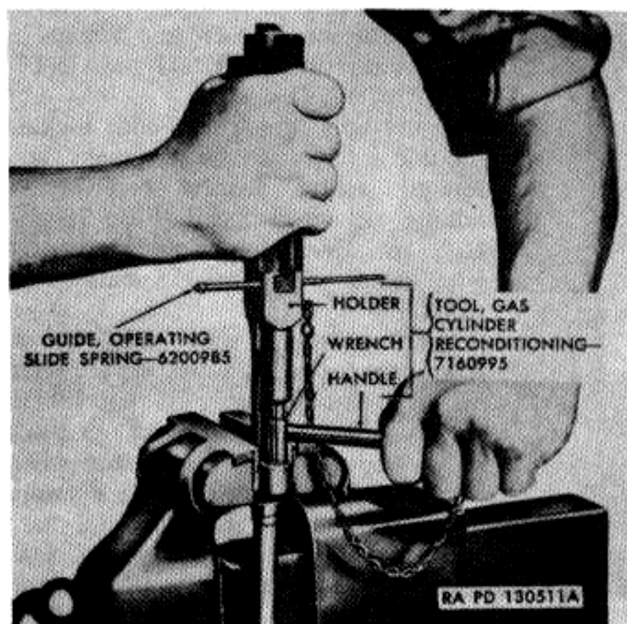
Figure 77. Removing piston nut from gas cylinder.
