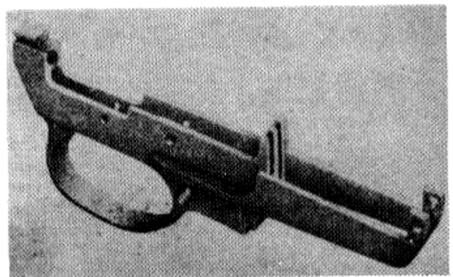
Figure 37. Trigger housing group parts.
