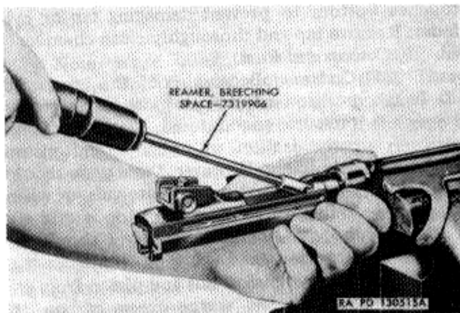
Figure 84. Reaming chamber for head space.
