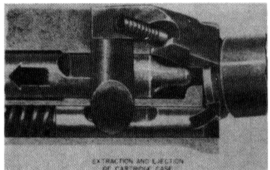
Figure 41. Extraction and ejection.
