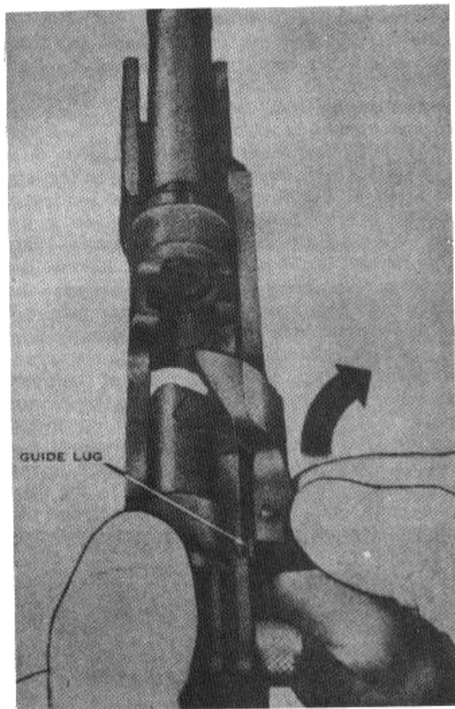
Figure 12-A. Removing the operating slide.
