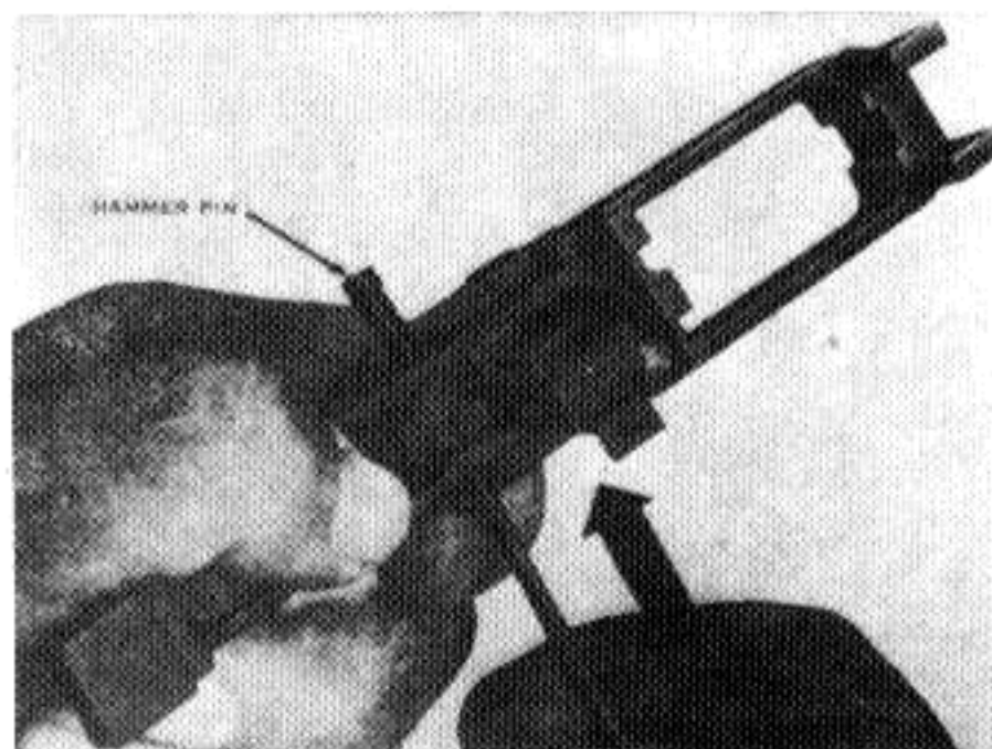
Figure 20. Removing the hammer pin.
