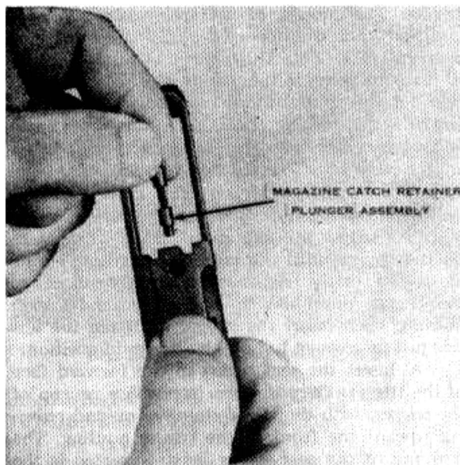
Figure 24-A. Removing the magazine catch retainer plunger assembly.
